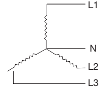
Three-Phase star; Four-wire; non-earthed neutral
